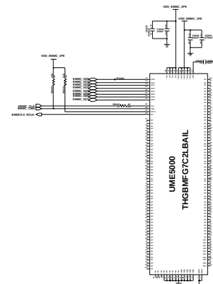
16GB eMMC 5.0 MLC
